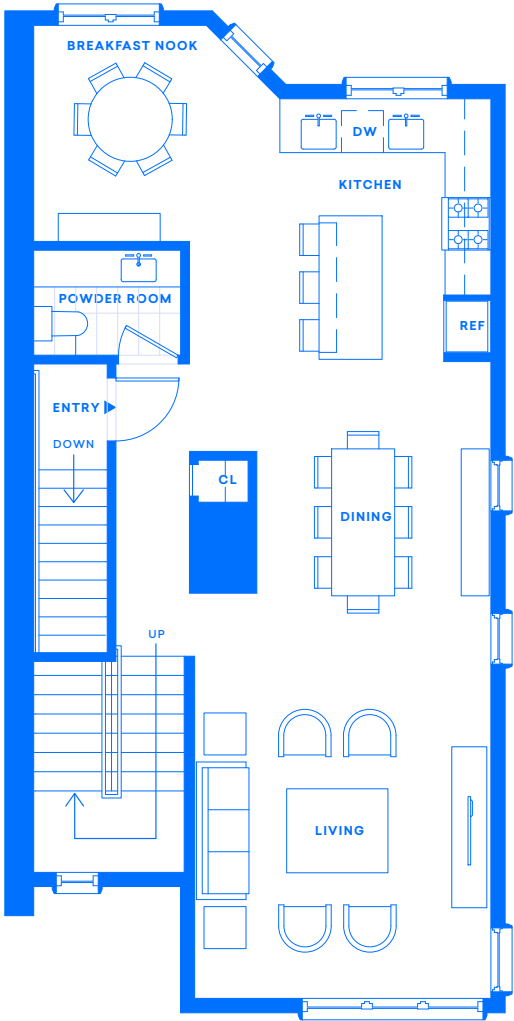
SECOND FLOOR
